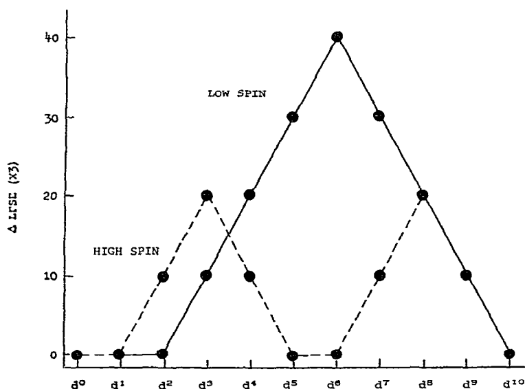
Fig. 4. Variation of \Delta LFSE with the d orbital occupation number, where \Delta LFSE = LFSE(\text{octahedron}) - LFSE(\text{trigonal prism}) .
