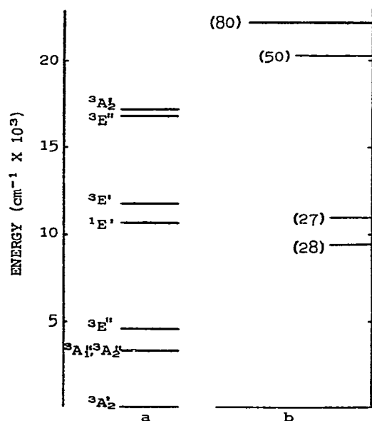
Fig. 11. Energy levels and spectrum of Ni(PccBF) 2+ . (a) Energy levels at \alpha = 0^\circ with Dq , B and C/B taken from Ni(bipy) 3 2+ . (b) The solution spectrum of Ni(PccBF)BF 4 . Extinction coefficients are given in parentheses.
